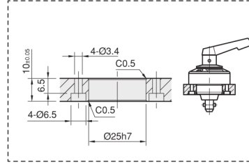
Product Nr. 1489 Single Touch Clamp • Black coating
