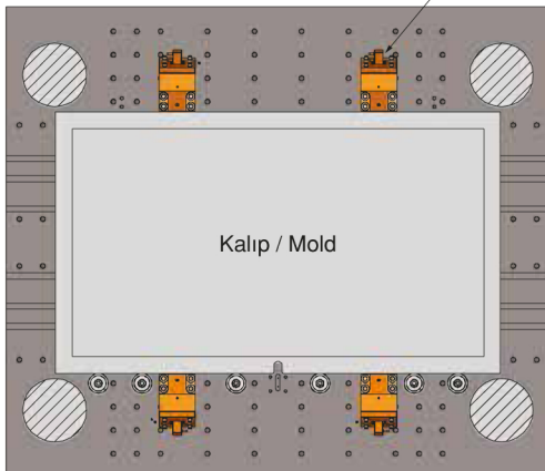
Hidrolik Pabuç Model CG Hydraulic Clamp Model CG
